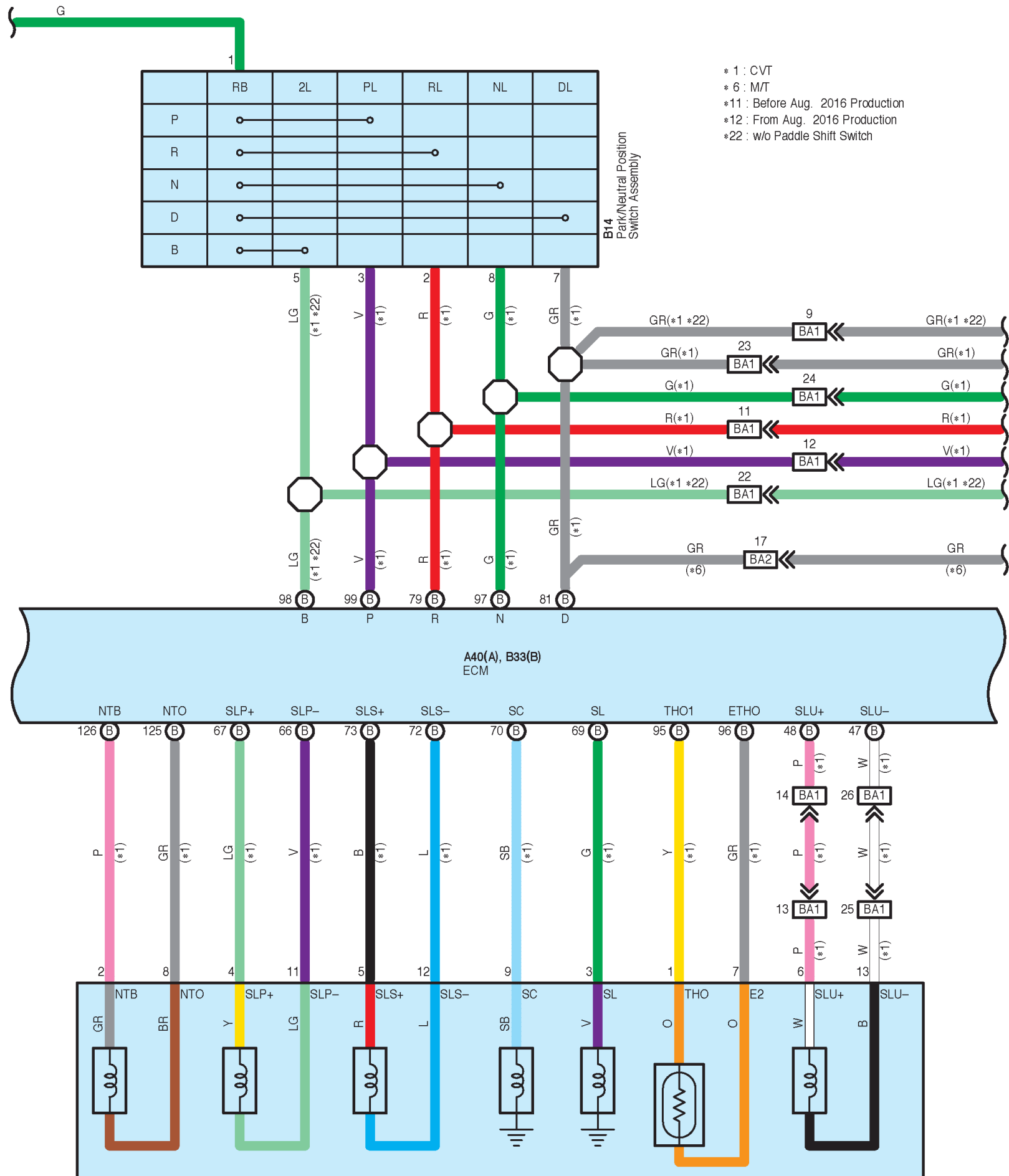
B18 CVT Solenoid (Transmission Wire)
